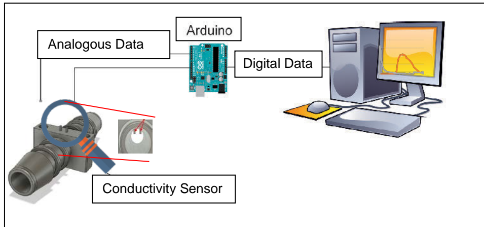
Figure 1: Conductivity sensor setup for data acquisition in a plug flow reactor. The sensor signal is transformed from analogous raw data via an Arduino microcontroller into a digital conductivity signal for further data analysis.
